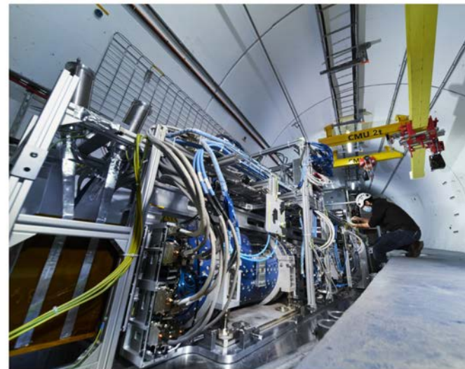
The FASER experiment in the LHC tunnel. (Image: CERN)
