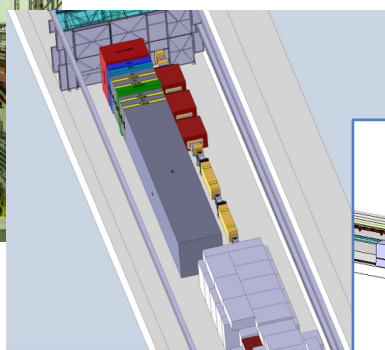
SHADOWS
