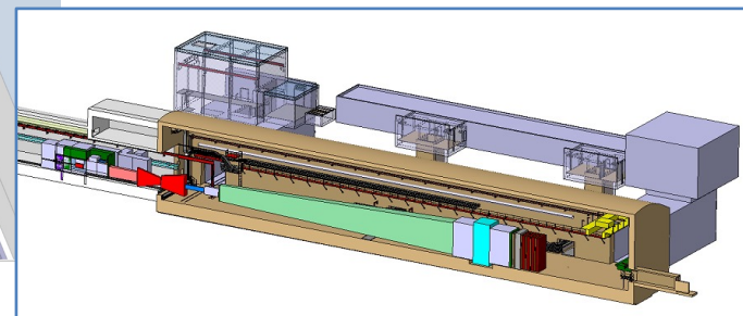
SHiP@ECN3
