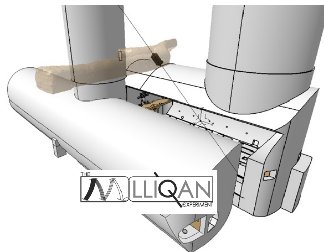
MilliQan Collaboration ( 2104.07151 )
